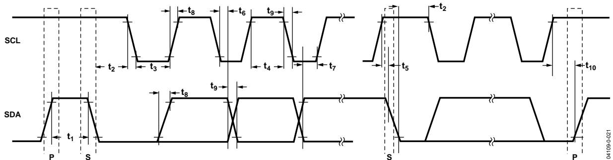
Figure 45. I 2 C Interface Detailed Timing Diagram
